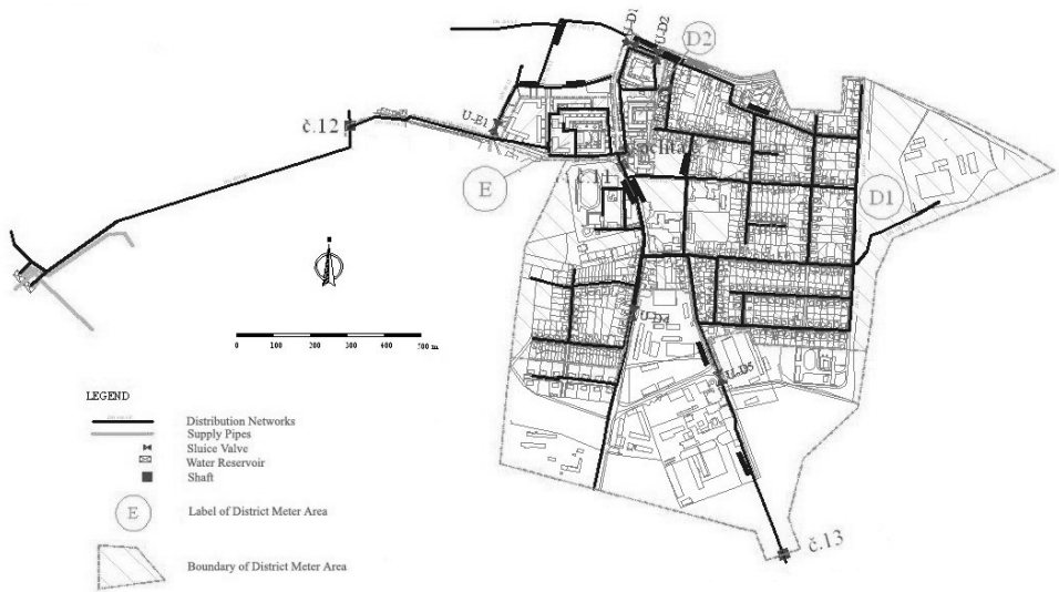
Fig. 3 District Meter Areas D_1 , D_2 and E
